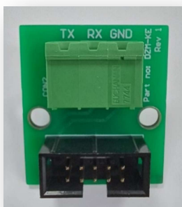
DZM-KE communication interface
