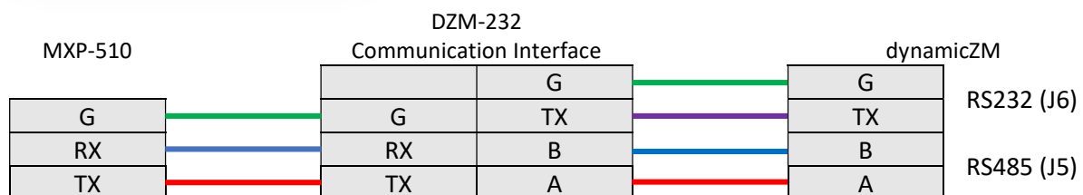
DZM-232 communication interface
