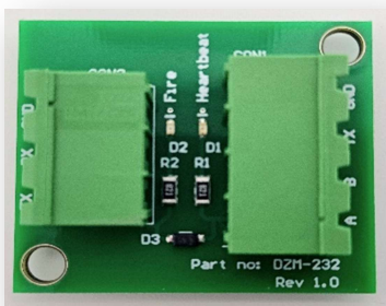
DZM-232 communication interface
